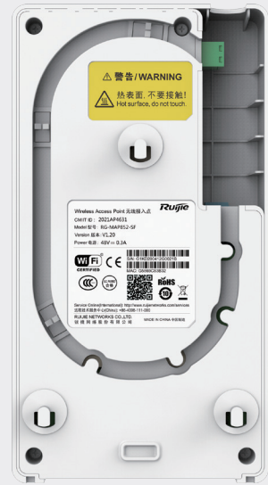
RG-MAP852-SF-S Rear View
